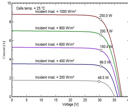
I-V Curve of 250W at 25°C cell temp. and different Irradiance level
