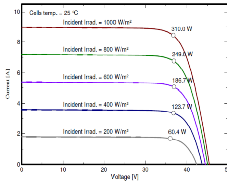
I-V Curve of 310W at 25°C cell temp. and different Irradiance level
